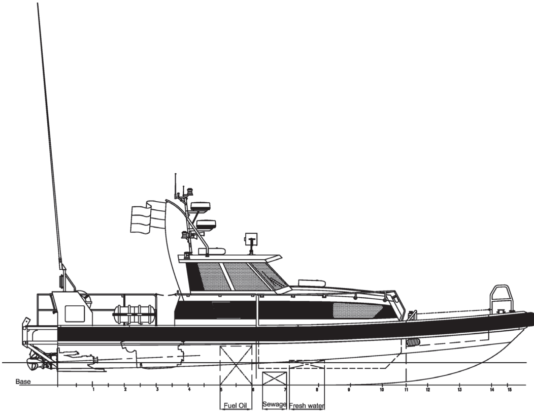
PROFILE
