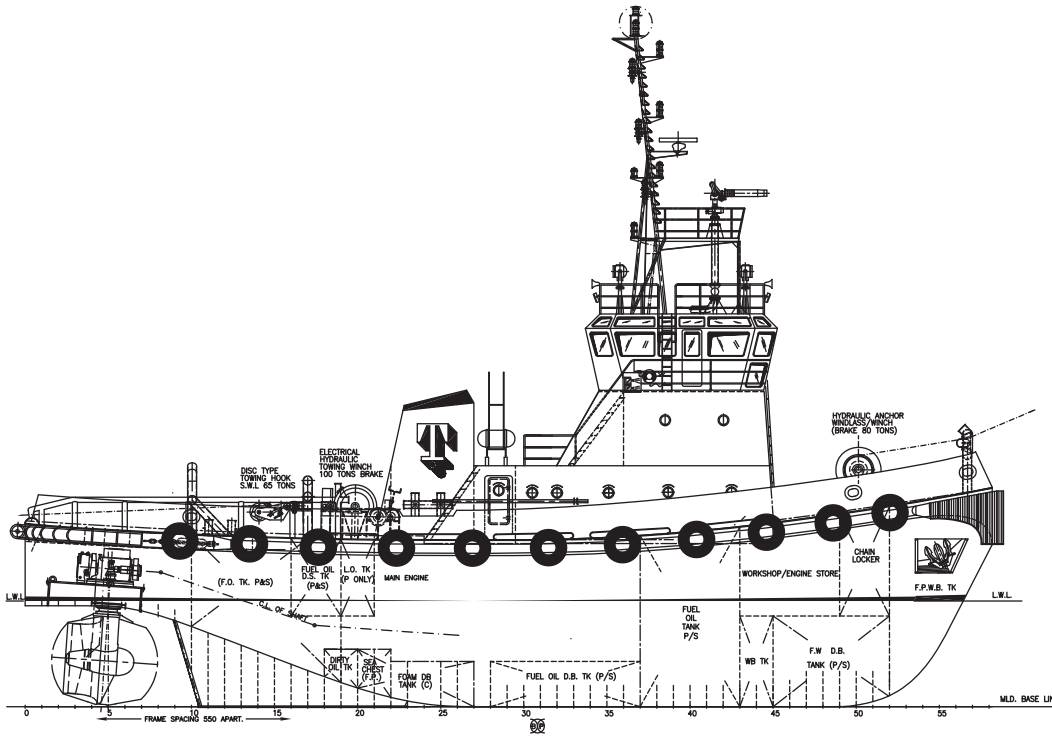
OUTBOARD PROFILE
