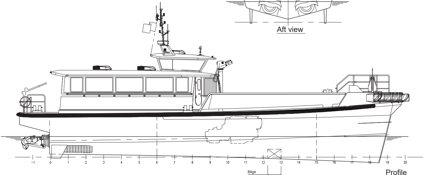
Profile
